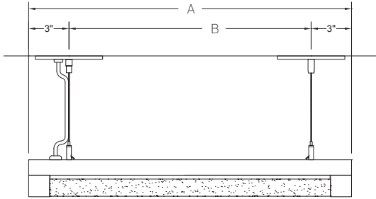
Side View - Cable Mount Single Fixture Option
