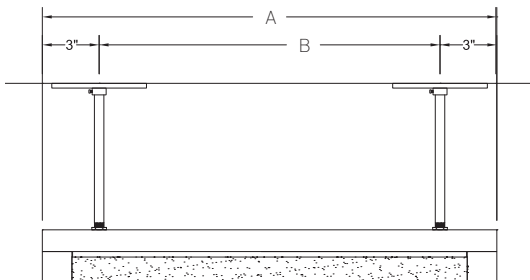
Side View - Pendant Mount Single Fixture Option
