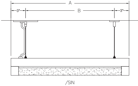
Side View - Cable Mount Continuous Run Option
