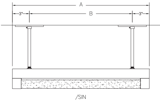
Side View - Pendant Mount Continuous Run Option
