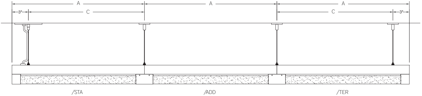
Side View - Pendant Mount Single Fixture Option
